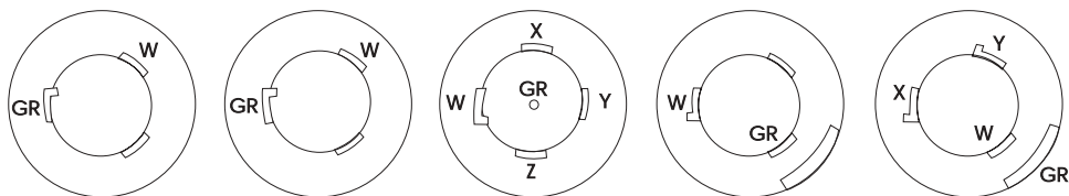
20 A 125V 2-POLE, 3-WIRE NEMA L5-20
